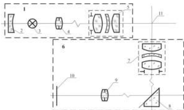
Figure 3. Optical Scheme of the Spectrometer "Masnik-A" 1-illuminating; 2-spherical mirror; 3-lamp lighting; 4,9- condenser with integrated field diaphragm; 5,7- projection lenses; 6-photometer; 8-mirror flat; 10- sensitive area of the photo detector; 11-space of work volume.
