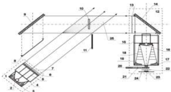
Figure 1. Optical Scheme of OMU Measurer of Spectral Transparency of the Atmosphere
