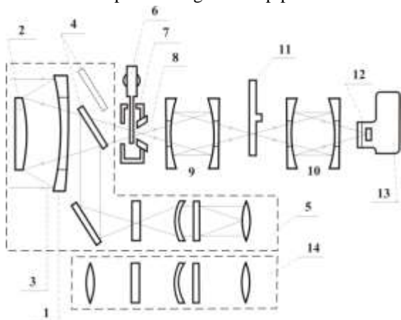
Figure 2. OMB Optical Scheme
